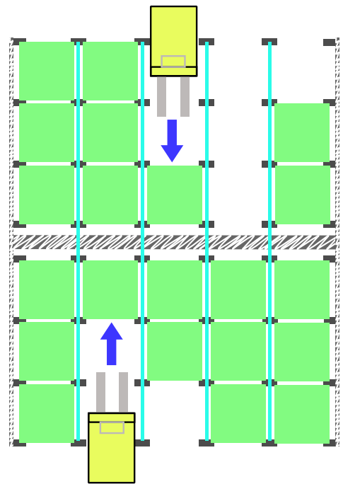
DRIVE-IN: dybdestablingsreol opstillet ryg mod ryg
